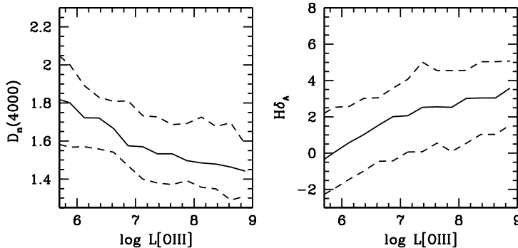
Figure 12: D_n(4000) and H\delta_A are plotted as a function of \log L[\text{OIII}] . The solid line shows the median, while the dashed lines indicate the 16-84 percentiles of the 1/V_{max} weighted distribution.
